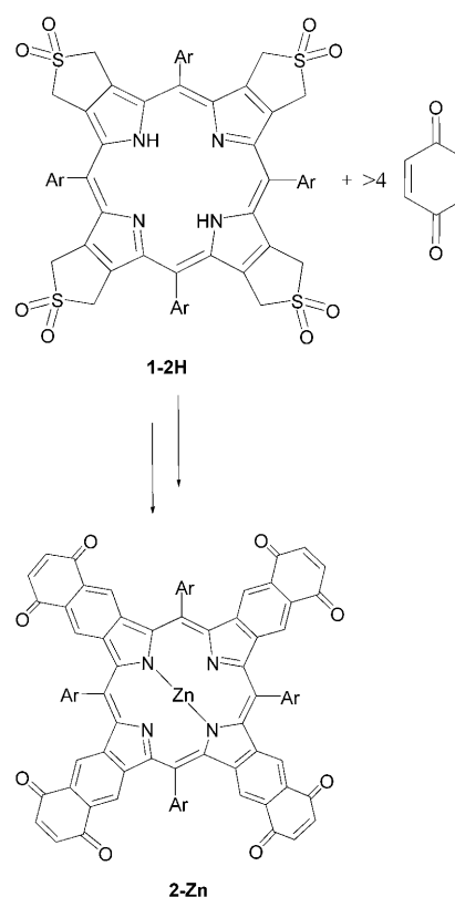
Scheme 1. Synthesis of the zinc tetraquinonoporphyrin 2-Zn . Ar = 3,5-di- tert -butylphenyl.
