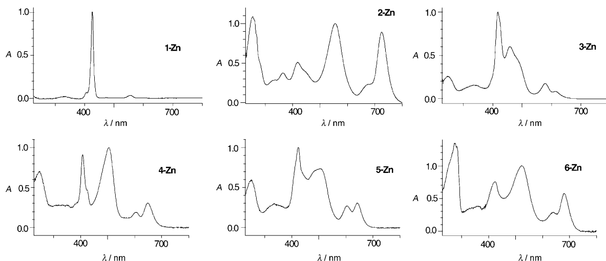
Figure 2. Effect of \beta,\beta' -bound quinone substituents. UV/Vis spectra of 1-Zn and of 2-Zn to 6-Zn in CH 2 Cl 2 (absorption not normalized; visible range (400–700 nm) highlighted).
