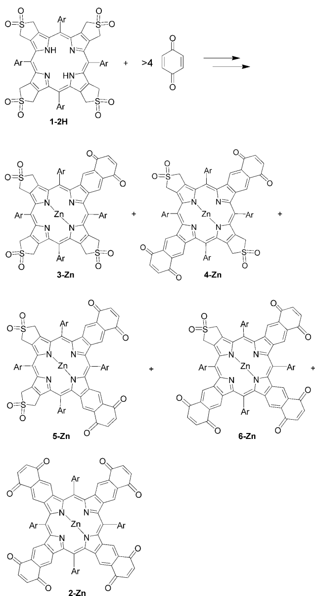
Scheme 2. Synthesis of the zinc \beta,\beta' -quinonoporphyrins 2-Zn to 6-Zn . Ar = 3,5-di- tert -butylphenyl.
