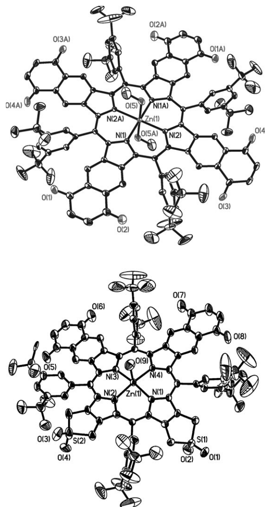
Figure 1. X-ray crystal structures of zinc tetraquinonoporphyrin 2-Zn (top) and of the “lateral” zinc bisquinonoporphyrin 5-Zn (bottom). (ORTEP plots; H atoms are omitted for clarity).
